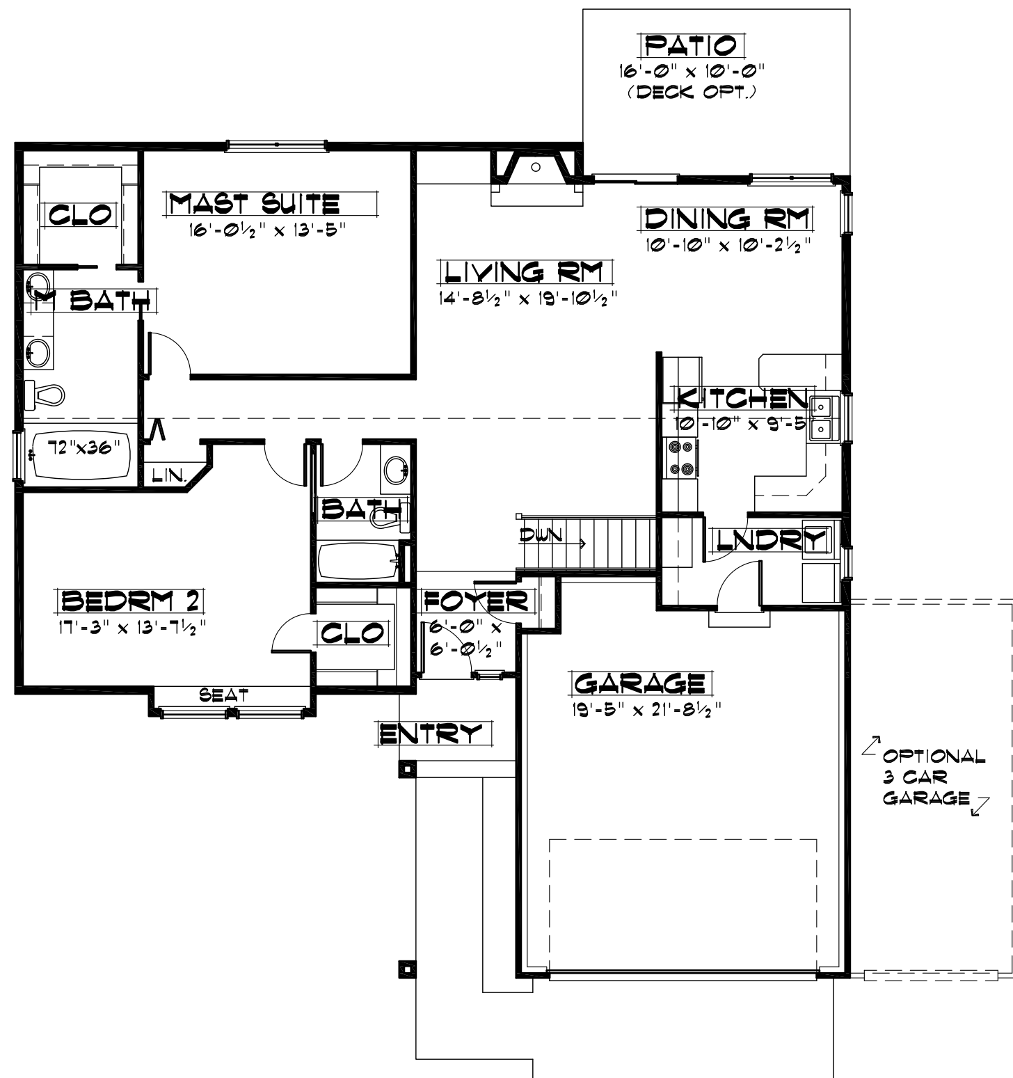
2 BR 50' Wide - Main Level Floor Plan 1,518 sq. ft.
